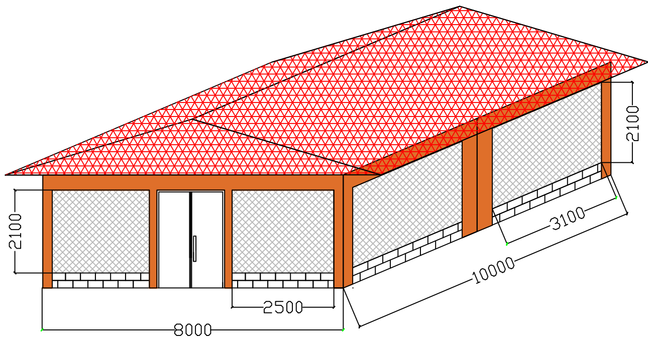
PERSPECTIVE PLAN
